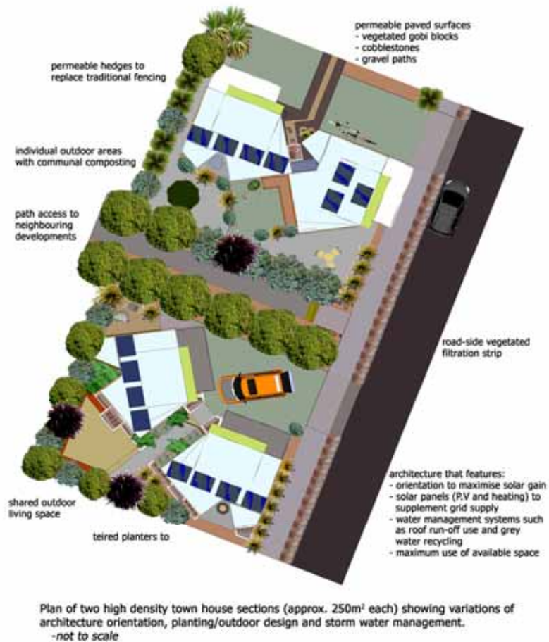
Figure 6: Concept plan and cross-section of the two high density town house sections for Liffey Spring Subdivision, Lincoln, South Island, New Zealand. Design: Jason Collett, 2007
