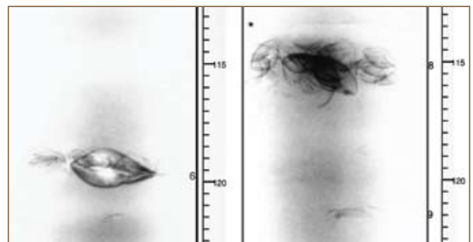
Positive renderings of x-rays of a cockle ( Austrovenus stuchburyi ) from c. 1200 mm below the sediment–water interface in Lake Waihola, Otago. Shells were carbon 14 dated as c. 4000 years old.
