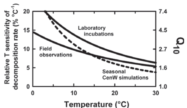
FIGURE 3 Relative temperature sensitivity based on field measurement, laboratory incubations, and CenW simulations with the temperature dependence from lab incubations but seasonally varying substrate availability.
