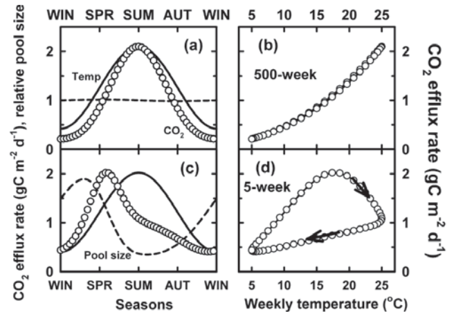
FIGURE 1 Simulated respiration rates (o) using a one-pool model, as a function of time (a, c) or temperature (b, d) for recalcitrant (a, b) or labile organic matter (c, d), with turn-over times given in the Figure. The dashed lines in (a, c) show changes in relative pool sizes, and solid lines show relative temperature.
