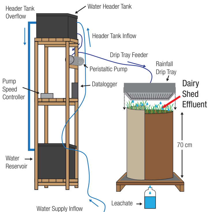
FIGURE 2 Experimental set-up.
