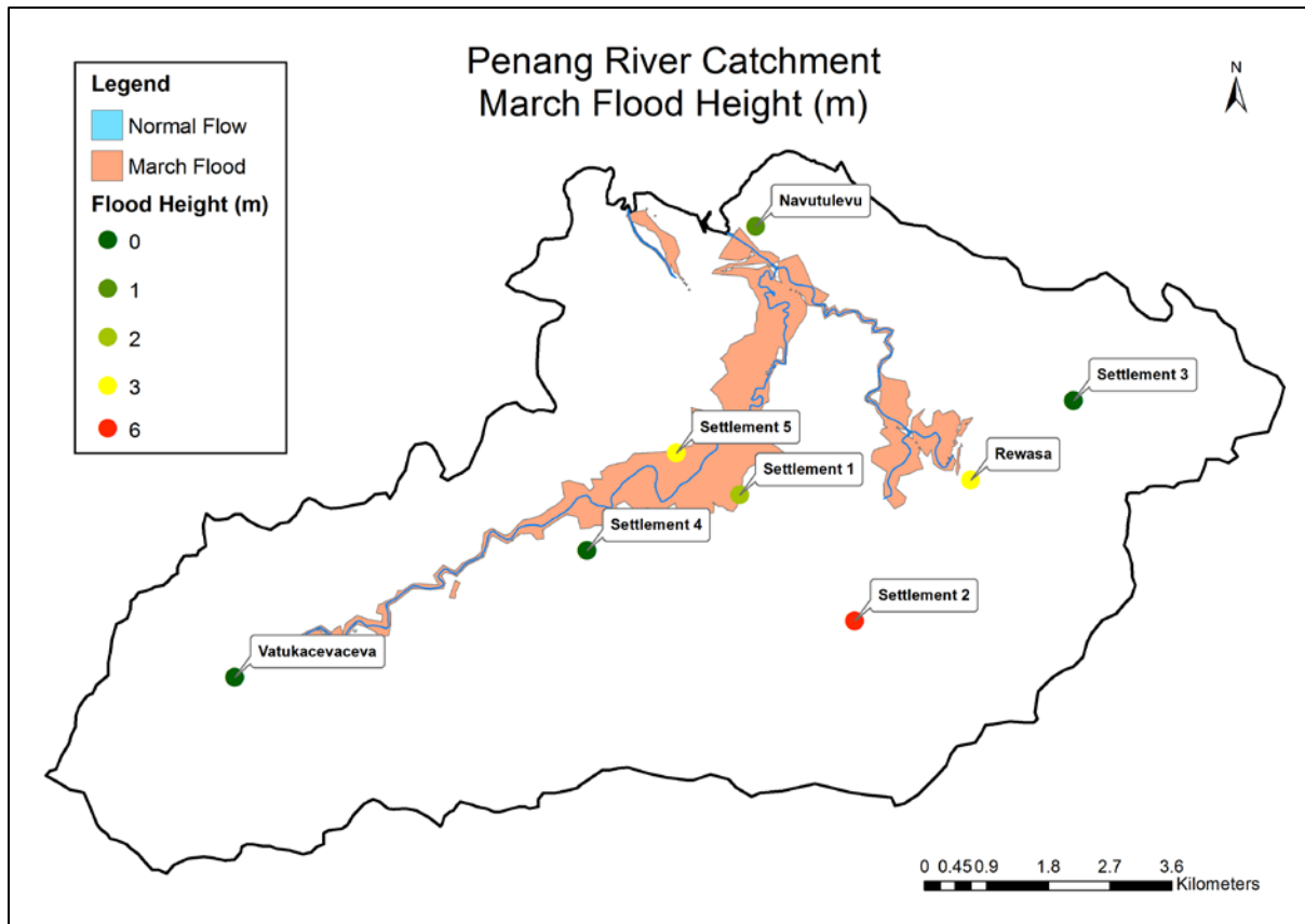
Figure 14. Modelled March 2012 flood height, Penang River catchment
