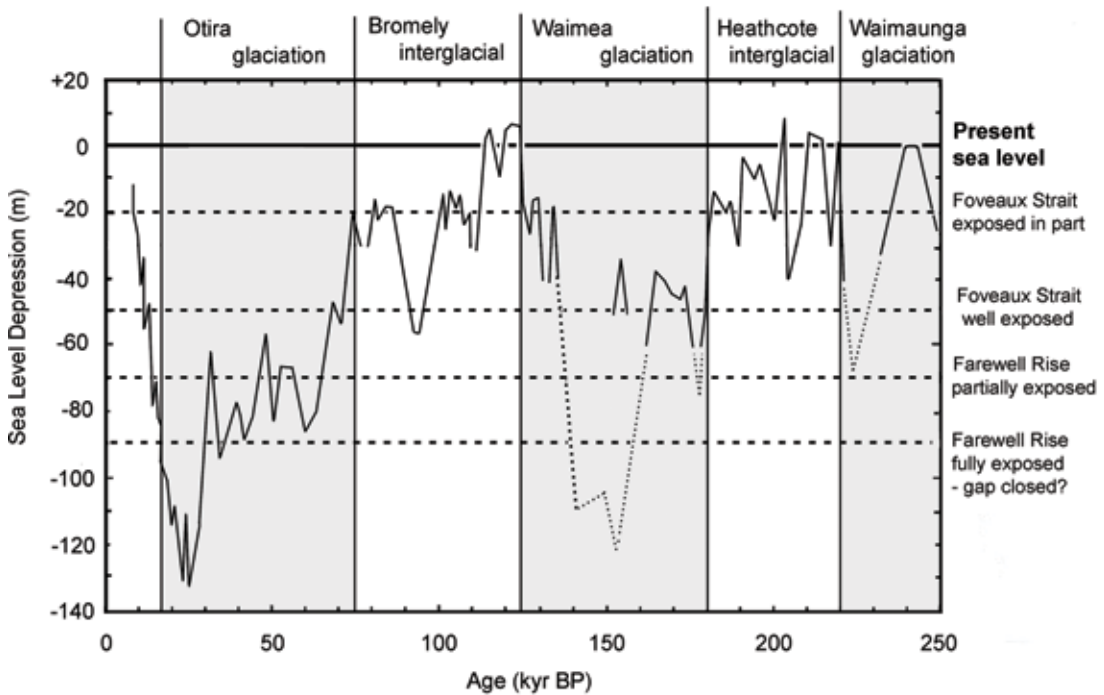
Fig. 515 Sea levels during the last 250 000 years BP in relation to possible exposure of Foveaux Strait and Farewell Rise (Cook Strait) during glacial and interglacial periods. Fine solid line = sea level curve, adapted from Thompson & Goldstein (2006). Fine dotted line = sea level estimates from Huybrecht (2002).
